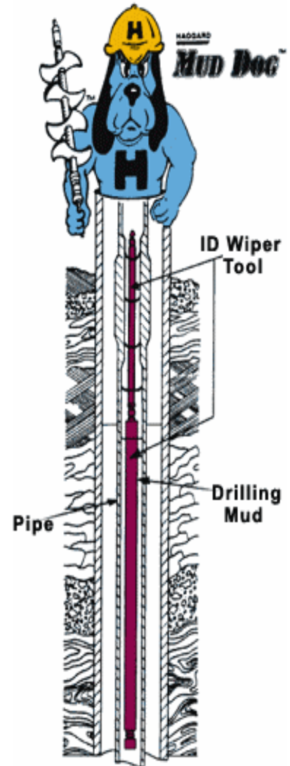
The HAGGARD MUD DOG ID WIPER At work in drill pipe
